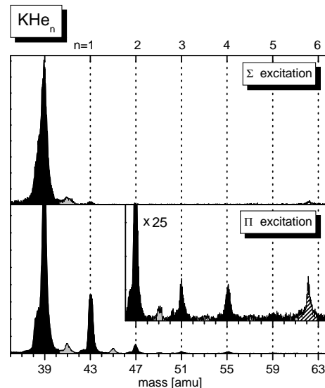
FIG. 1: Mass spectrum from photo-ionization of potassium-doped helium nanodroplets with a pair of femtosecond laser pulses separated by 100 ps. The spectrum in the upper panel is recorded at a photon energy of 12990 \text{ cm}^{-1} ; in the lower panel, exciting at 12900 \text{ cm}^{-1} , exciplex formation is observed. The peak at mass 62 is due to \text{KNa} molecules. The peaks shaded in gray correspond to ^{41}\text{K} and its exciplexes.
